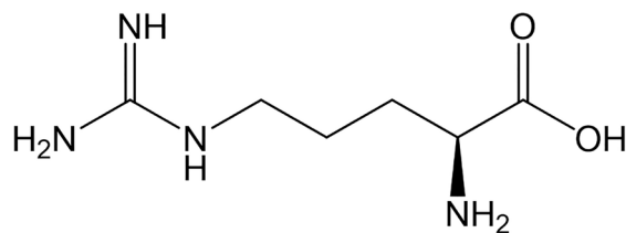
Figure 1. Arginine
