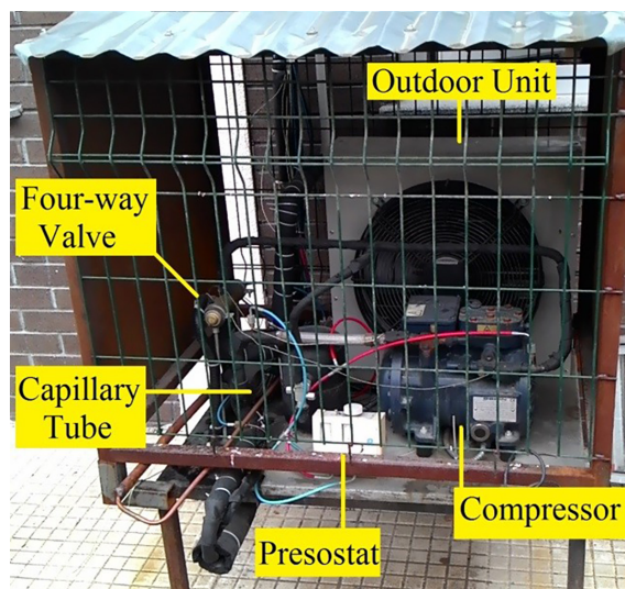
Figure 3. Outdoor unit of the heat pump
